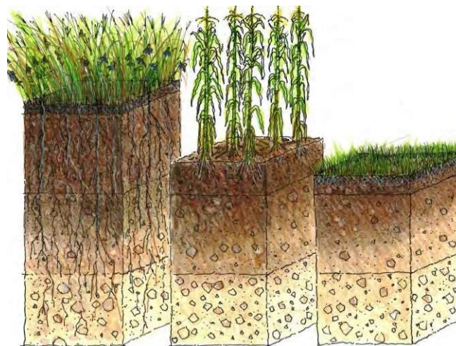
Figure C5-S6- 1: (L to R) Prairie soil profile, soils under modern agriculture and soils after urban development under turf grass.
